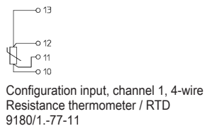
Connection diagram 9180/1.-77-11
