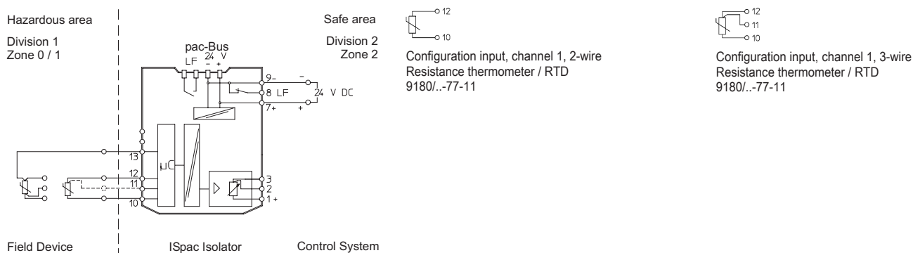
Connection diagram 9180/1.-77-11
