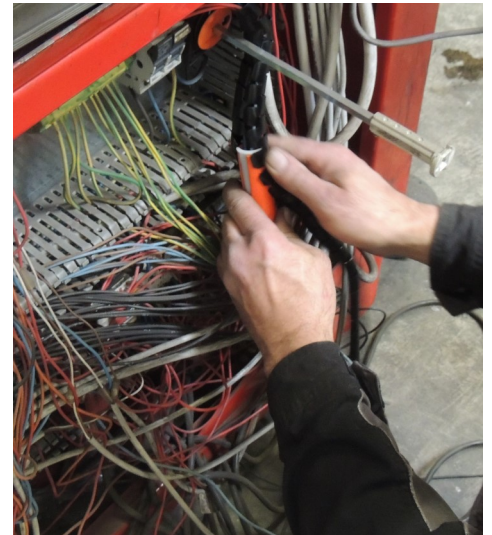
3 Hold the sheath with one hand and slide the tool: the cables are "swallowed" by the sheath.
